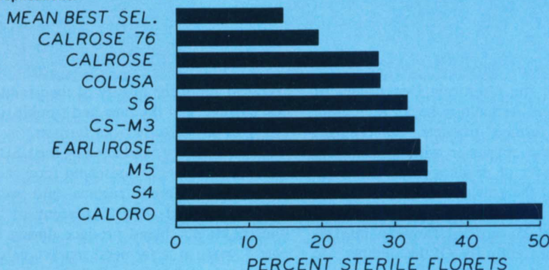
Fig. 3. Percent sterile florets of nine standard cultivars compared with the mean of the best 10 percent of 100 cultivars and selections. The sterility figures are means of five tests conducted from 1974 to 1976 at Davis and one test in Hawaii in 1975-76.
