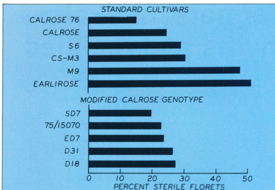
Fig. 2. Percent sterile florets of standard cultivars and modified Calrose genotypes grown at Davis, 1976. Sterility figures are means of two planting dates (May 1 and May 19), each with 12 replications.
