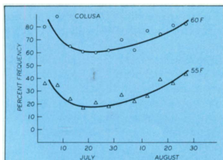
Fig. 1. Percent frequency of occurrence of minimum temperatures of 60° F and below and 55° F and below at Colusa, based on records from 1958 to 1977.
