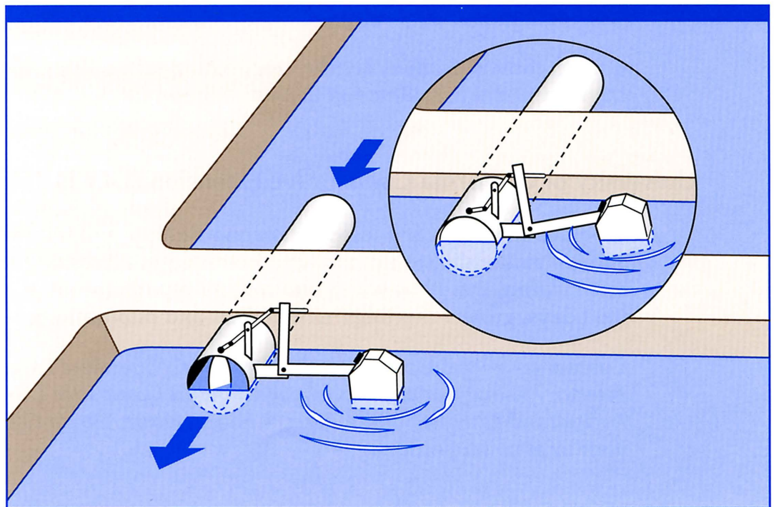
FIGURE 8. Close up of a float-valve rice box between two basins.
